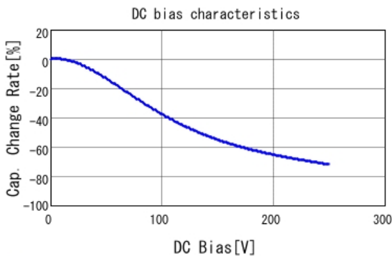
■ GRM21AR72E332KW01 C-DC bias capchange, 25.0degC, AC1V
