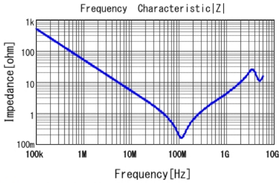
■ GRM21AR72E332KW01 |Z| DCOV, 25degC
