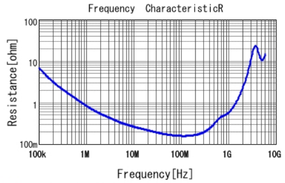
■ GRM21AR72E332KW01 R DCOV, 25degC
