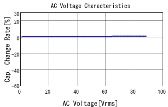
■ GRM21AR72E332KW01 C-AC Voltage capchange, DCOV, 25.0d
