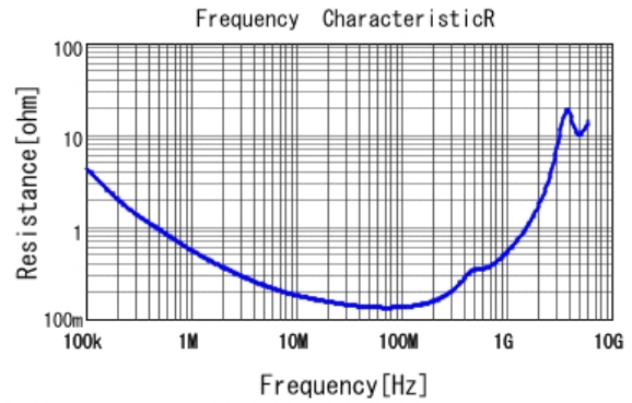
■ GRM21AR72E472KW01 R DCOV, 25degC
