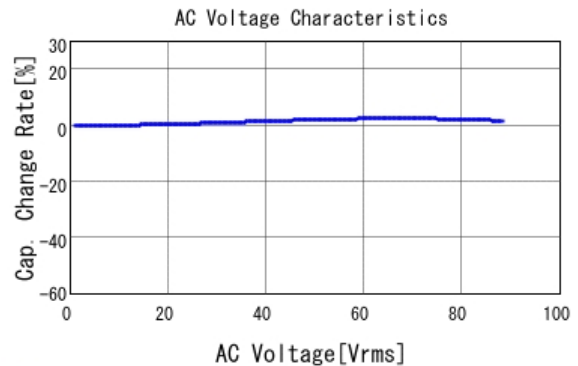
■ GRM21AR72E472KW01 C-AC Voltage capchange, DCOV, 25.0d
