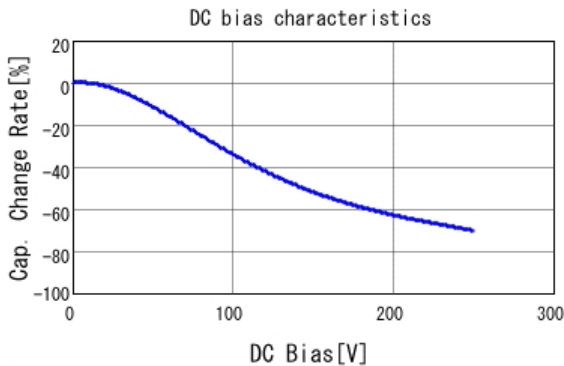
■ GRM21AR72E472KW01 C-DC bias capchange, 25.0degC, AC1V
