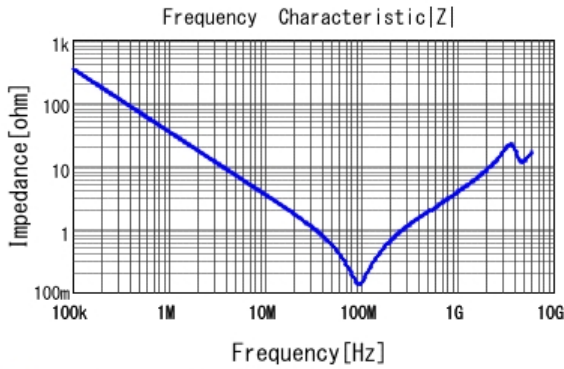
■ GRM21AR72E472KW01 |Z| DCOV, 25degC
