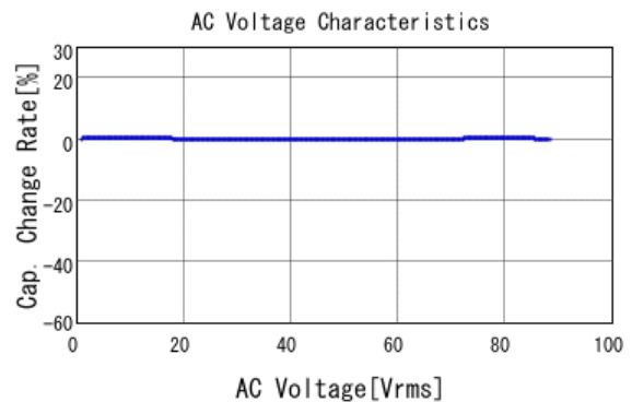
■ GRM21AR72E682KW01 C-AC Voltage capchange, DCOV, 25.0d
