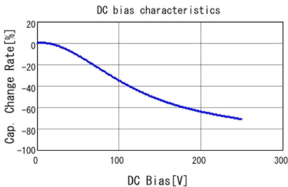
■ GRM21AR72E682KW01 C-DC bias capchange, 25.0degC, AC1V
