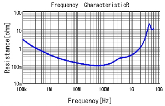
■ GRM21AR72E682KW01 R DCOV, 25degC
