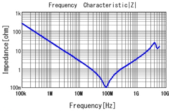
■ GRM21AR72E682KW01 |Z| DCOV, 25degC
