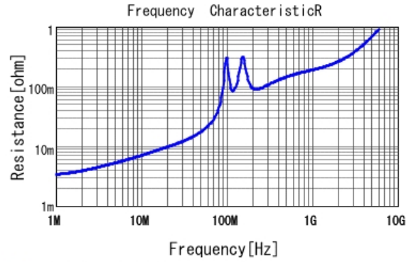
■ GRM21B5C1H183JA01 R DCOV, 25degC
