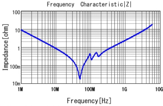
■ GRM21B5C1H183JA01 |Z| DCOV, 25degC
