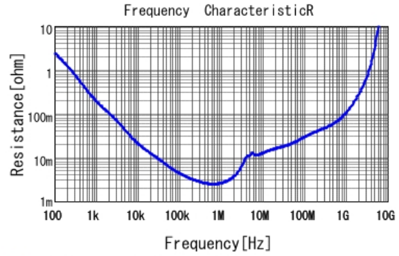
■ GRM21BB31A106KE18 R DCOV, 20degC
