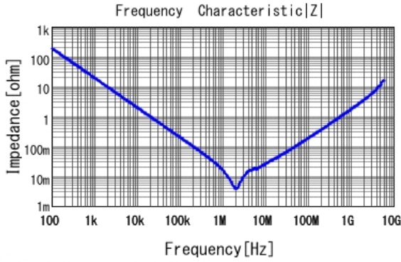
■ GRM21BB31A106KE18 |Z| DCOV, 20degC
