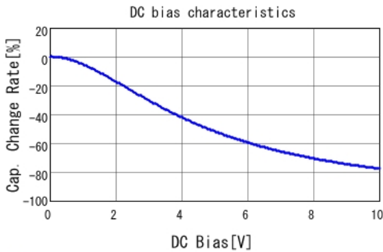
■ GRM21BB31A106KE18 C-DC bias capchange, 20.0degC, AC0.
