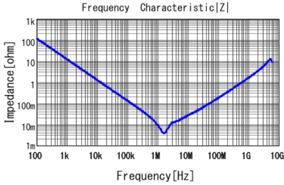
■ GRM21BC80G226ME39 |Z| DCOV, 25degC
