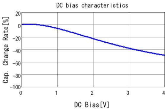
■ GRM21BC80G226ME39 C-DC bias capchange, 25.0degC, AC0.
