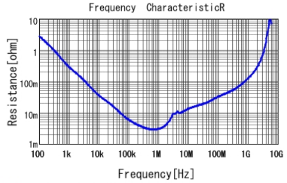
■ GRM21BC80G226ME39 R DCOV, 25degC
