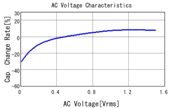
■ GRM21BC80G226ME39 C-AC Voltage capchange, DCOV, 25.0d
