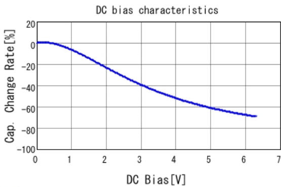
■ GRM21BC80J226ME51 C-DC bias capchange, 25.0degC, AC0.
