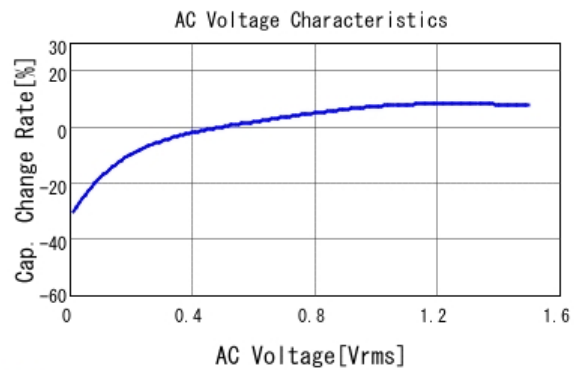
■ GRM21BC80J226ME51 C-AC Voltage capchange, DCOV, 25.0d
