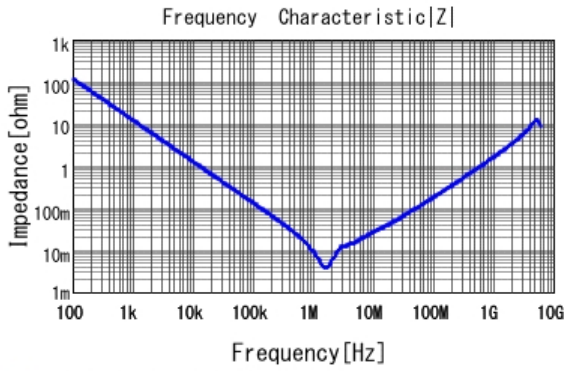
■ GRM21BC80J226ME51 |Z| DCOV, 25degC
