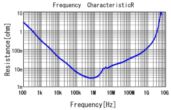
■ GRM21BC80J226ME51 R DCOV, 25degC
