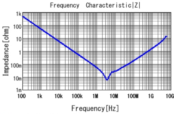
■ GRM21BC81E475KA12 |Z| DCOV, 25degC
