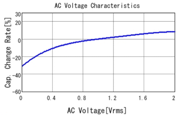
■ GRM21BC81E475KA12 C-AC Voltage capchange, DCOV, 25.0d
