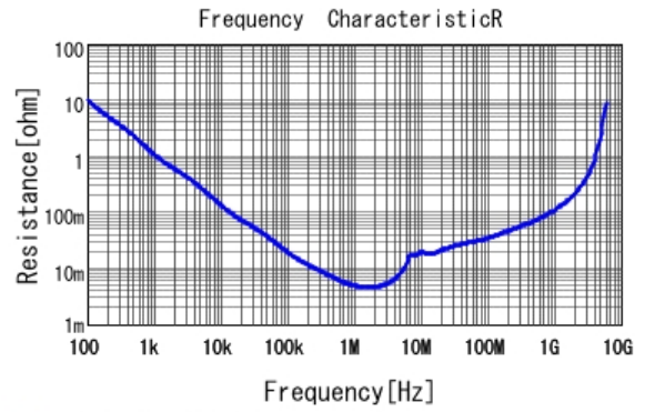
■ GRM21BC81E475KA12 R DCOV, 25degC
