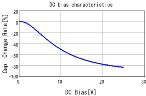
■ GRM21BC81E475KA12 C-DC bias capchange, 25.0degC, AC1.
