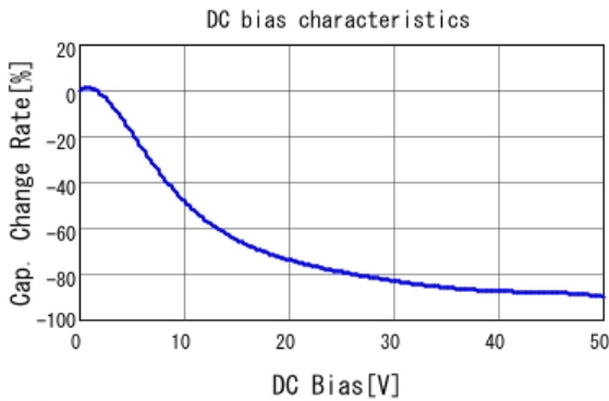
■ GRM21BC81H475KE11 C-DC bias capchange, 25.0degC, AC1V
