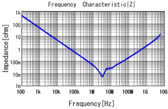
■ GRM21BC81H475KE11 |Z| DCOV, 25degC
