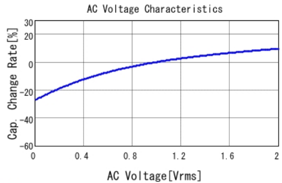
■ GRM21BC81H475KE11 C-AC Voltage capchange, DCOV, 25.0d
