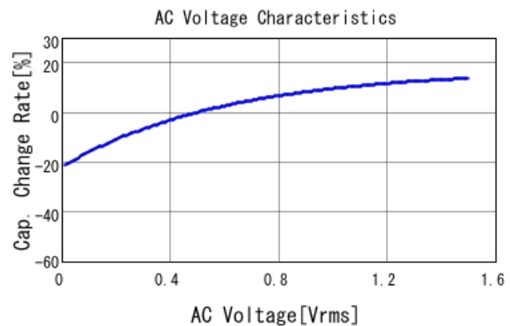
■ GRM21BR60J106KE19 C-AC Voltage capchange, DCOV, 25.0d
