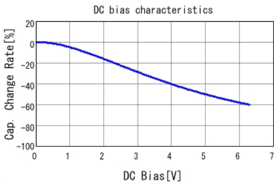
■ GRM21BR60J106KE19 C-DC bias capchange, 25.0degC, AC0.
