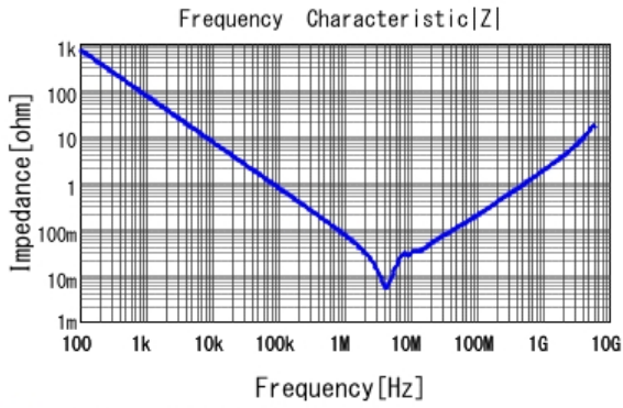
■ GRM21BR60J225KA01 |Z| DCOV, 25degC
