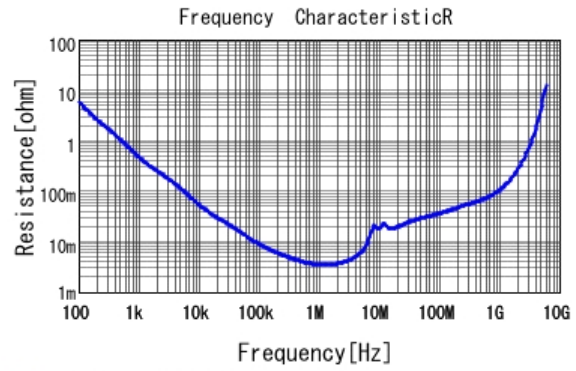
■ GRM21BR60J225KA01 R DCOV, 25degC
