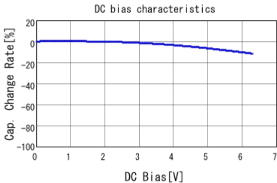
■ GRM21BR60J225KA01 C-DC bias capchange, 25.0degC, AC1.
