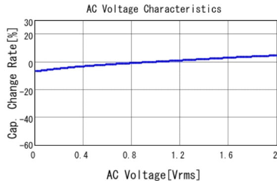
■ GRM21BR60J225KA01 C-AC Voltage capchange, DCOV, 25.0d
