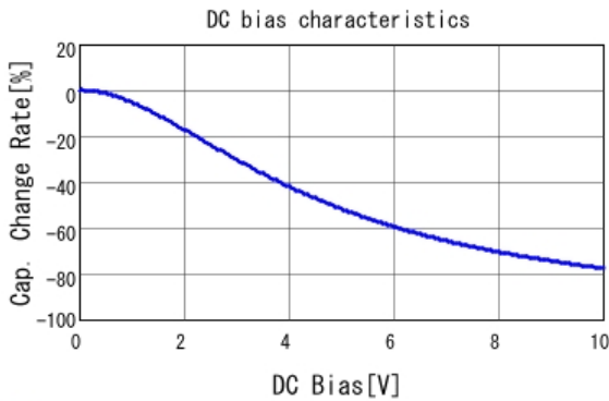
■ GRM21BR61A106ME19 C-DC bias capchange, 25.0degC, AC0.
