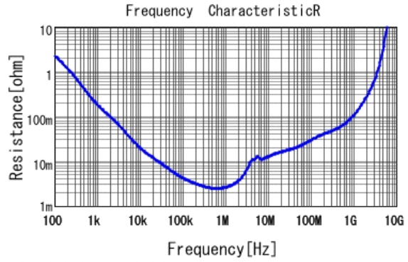
■ GRM21BR61A106ME19 R DCOV, 25degC
