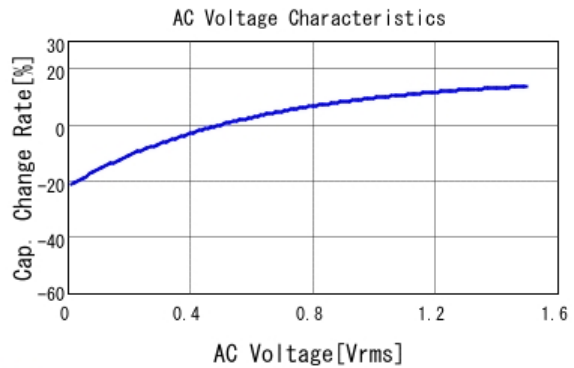
■ GRM21BR61A106ME19 C-AC Voltage capchange, DCOV, 25.0d
