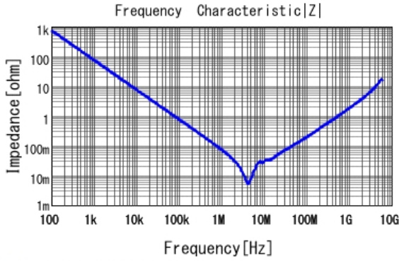
■ GRM21BR61A225KA01 |Z| DCOV, 25degC
