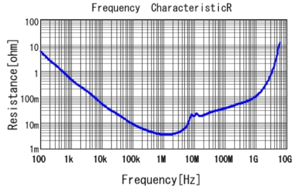
■ GRM21BR61A225KA01 R DCOV, 25degC
