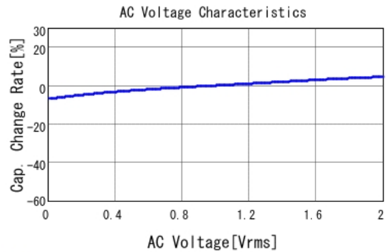
■ GRM21BR61A225KA01 C-AC Voltage capchange, DCOV, 25.0d
