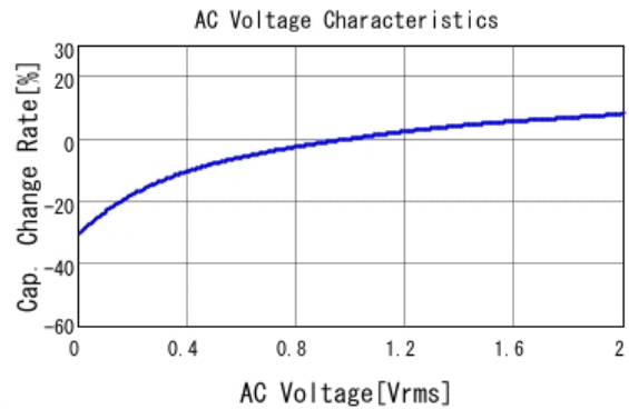
■ GRM21BR61A475KA73 C-AC Voltage capchange, DCOV, 25.0d
