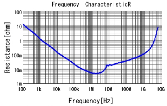
■ GRM21BR61A475KA73 R DCOV, 25degC
