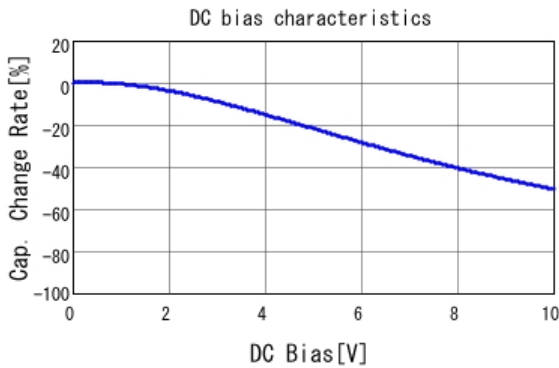
■ GRM21BR61A475KA73 C-DC bias capchange, 25.0degC, AC1.
