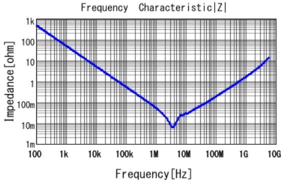
■ GRM21BR61A475KA73 |Z| DCOV, 25degC
