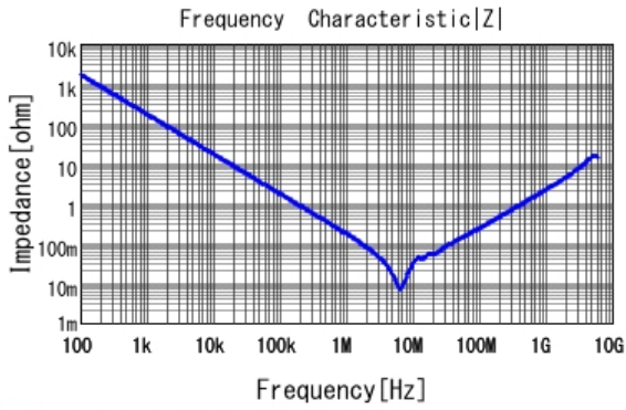
■ GRM21BR61C105KA01 |Z| DCOV, 25degC
