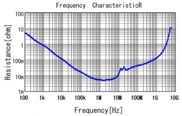
■ GRM21BR61C105KA01 R DCOV, 25degC
