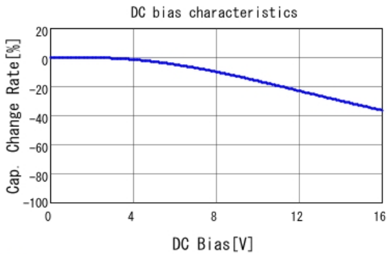
■ GRM21BR61C105KA01 C-DC bias capchange, 25.0degC, AC1.
