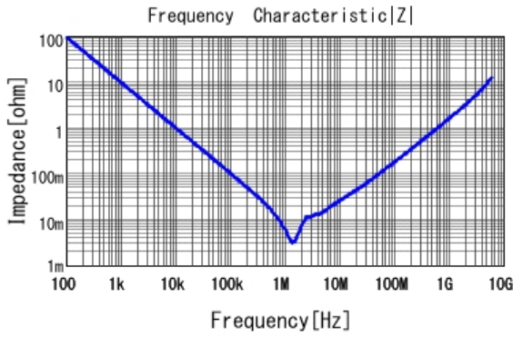
■ GRM21BR61C226ME44 |Z| DCOV, 25degC
