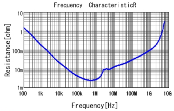
■ GRM21BR61C226ME44 R DCOV, 25degC
