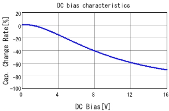
■ GRM21BR61C475KA88 C-DC bias capchange, 25.0degC, AC1.
