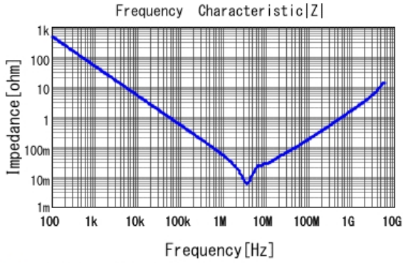
■ GRM21BR61C475KA88 |Z| DCOV, 25degC
