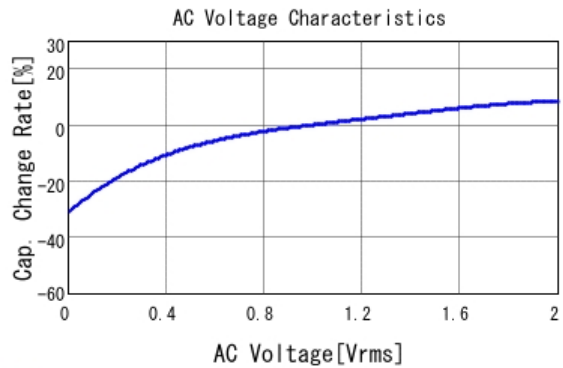
■ GRM21BR61C475KA88 C-AC Voltage capchange, DCOV, 25.0d
