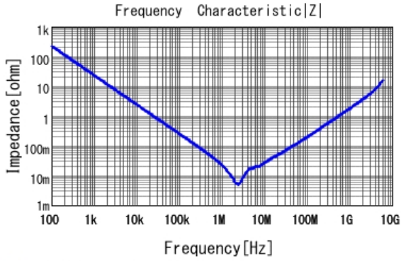
■ GRM21BR61D106KE15 |Z| DCOV, 25degC
