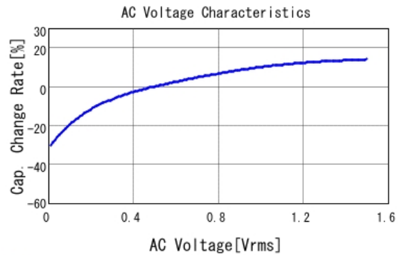
■ GRM21BR61D106KE15 C-AC Voltage capchange, DCOV, 25.0d
