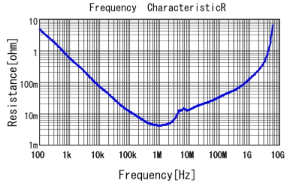
■ GRM21BR61D106KE15 R DCOV, 25degC
