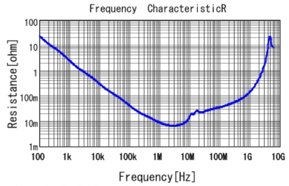
■ GRM21BR61E225KA12 R DCOV, 25degC
