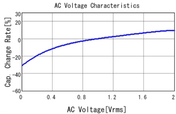
■ GRM21BR61E225KA12 C-AC Voltage capchange, DCOV, 25.0d
