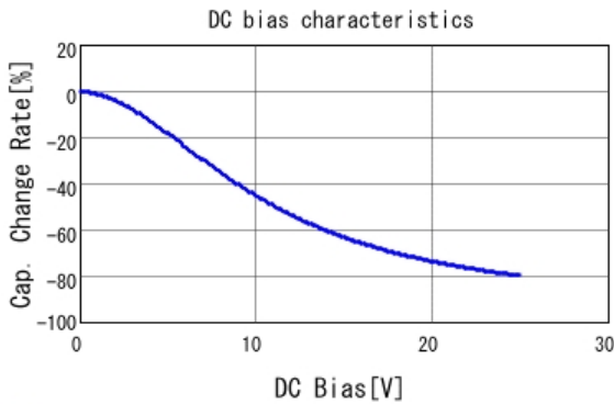
■ GRM21BR61E225KA12 C-DC bias capchange, 25.0degC, AC1.
