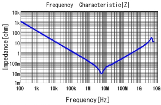
■ GRM21BR61E225KA12 |Z| DCOV, 25degC
