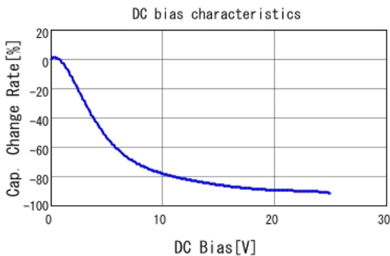
■ GRM21BR61E226ME44 C-DC bias capchange, 25.0degC, AC0.
