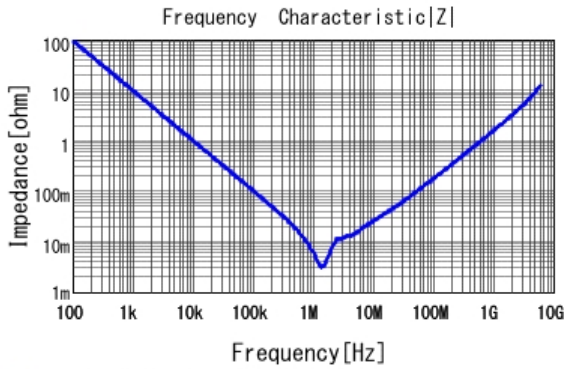
■ GRM21BR61E226ME44 |Z| DCOV, 25degC
