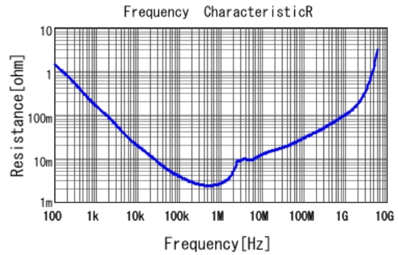
■ GRM21BR61E226ME44 R DCOV, 25degC
