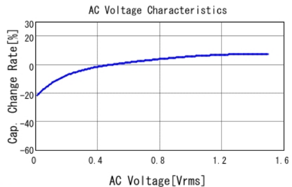
■ GRM21BR61E226ME44 C-AC Voltage capchange, DCOV, 25.0d
