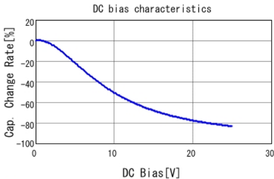
■ GRM21BR61E475KA12 C-DC bias capchange, 25.0degC, AC1.
