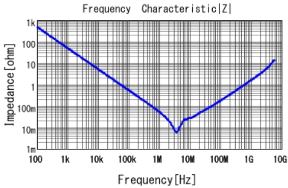
■ GRM21BR61E475KA12 |Z| DCOV, 25degC
