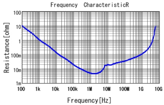
■ GRM21BR61E475KA12 R DCOV, 25degC
