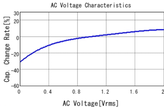
■ GRM21BR61E475KA12 C-AC Voltage capchange, DCOV, 25.0d
