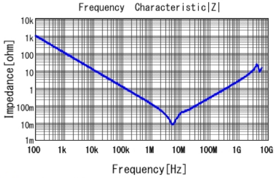
■ GRM21BR61H225KA73 |Z| DCOV, 25degC
