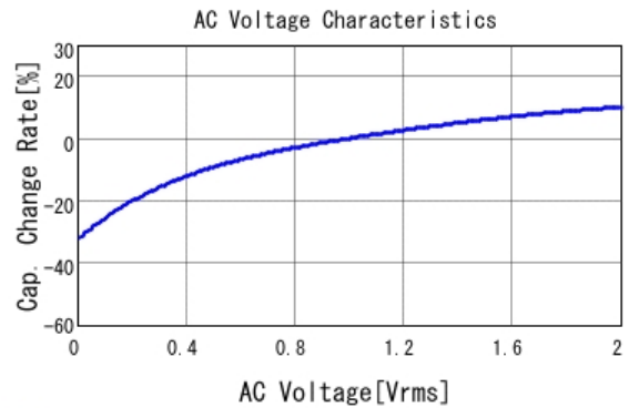
■ GRM21BR61H225KA73 C-AC Voltage capchange, DCOV, 25.0d
