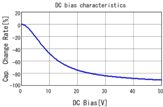
■ GRM21BR61H225KA73 C-DC bias capchange, 25.0degC, AC1.
