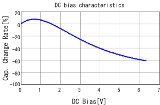
■ GRM21BR70J106KE76 C-DC bias capchange, 25.0degC, AC0.
