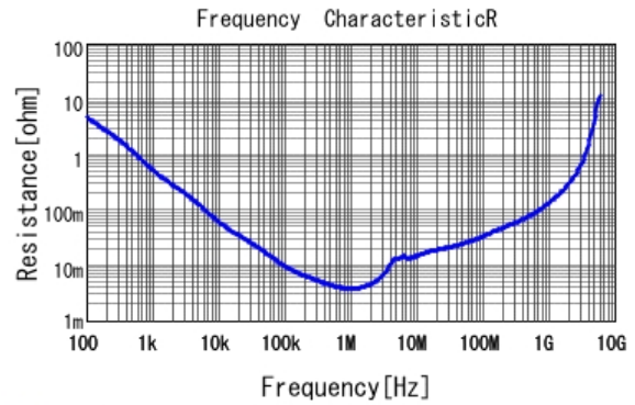
■ GRM21BR70J106KE76 R DCOV, 25degC
