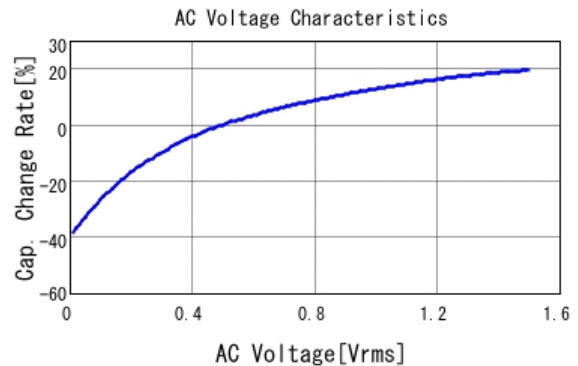
■ GRM21BR70J106KE76 C-AC Voltage capchange, DCOV, 25.0d
