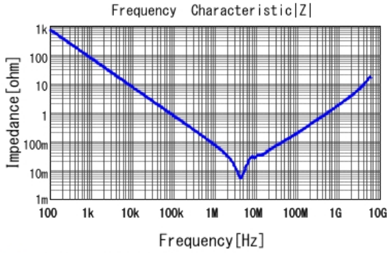
■ GRM21BR70J225KA01 |Z| DCOV, 25degC
