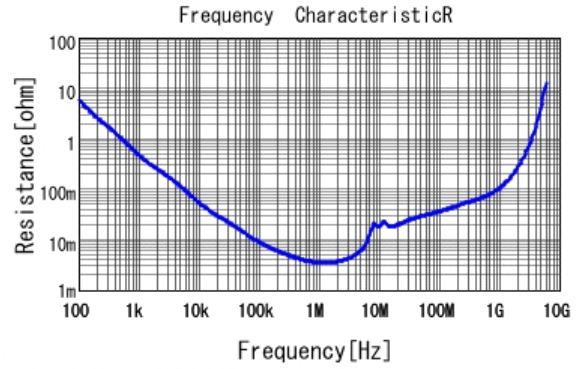
■ GRM21BR70J225KA01 R DCOV, 25degC
