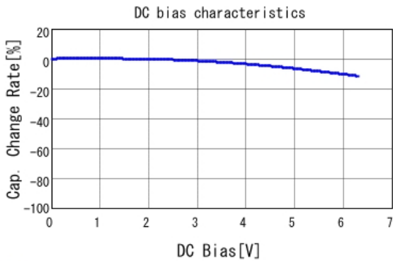
■ GRM21BR70J225KA01 C-DC bias capchange, 25.0degC, AC1.
