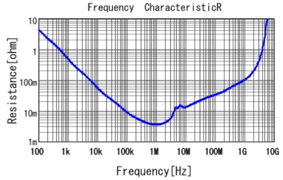
■ GRM21BR71A106KA73 R DCOV, 25degC
