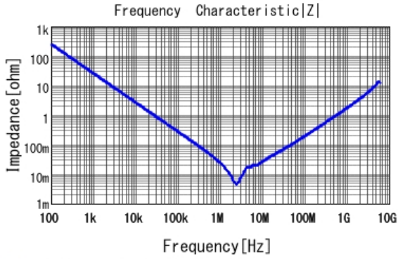
■ GRM21BR71A106KA73 |Z| DCOV, 25degC
