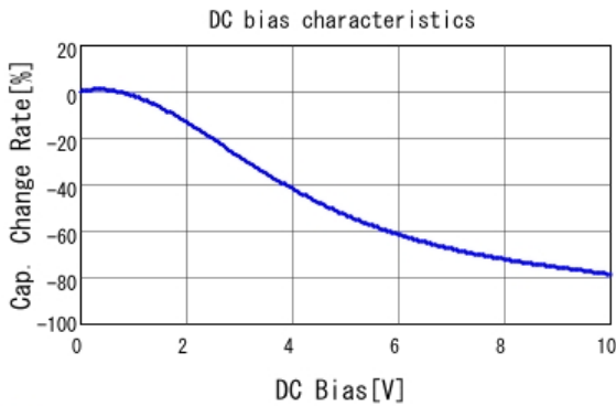
■ GRM21BR71A106KA73 C-DC bias capchange, 25.0degC, AC1V
