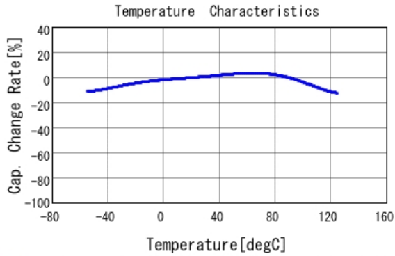
■ GRM21BR71A106KA73 C-Temp. capchange, DC0.0V, AC0.35Vr
