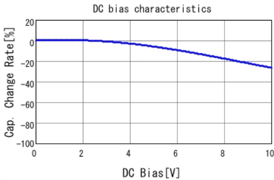
■ GRM21BR71A225KA01 C-DC bias capchange, 25.0degC, AC1.
