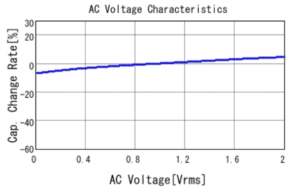
■ GRM21BR71A225KA01 C-AC Voltage capchange, DCOV, 25.0d
