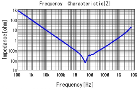
■ GRM21BR71A225KA01 |Z| DCOV, 25degC
