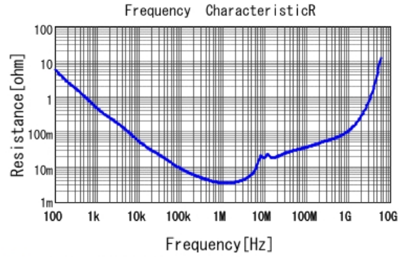
■ GRM21BR71A225KA01 R DCOV, 25degC
