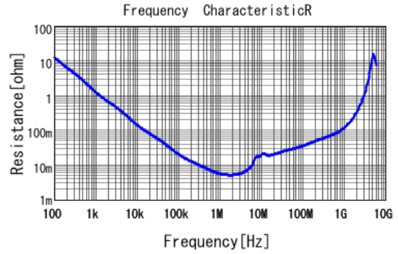
■ GRM21BR71A475KA73 R DCOV, 25degC
