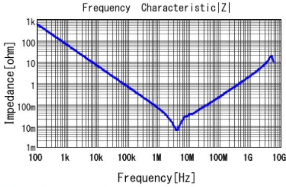
■ GRM21BR71A475KA73 |Z| DCOV, 25degC
