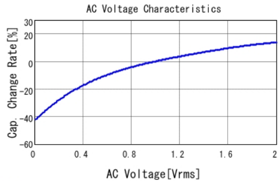
■ GRM21BR71A475KA73 C-AC Voltage capchange, DCOV, 25.0d
