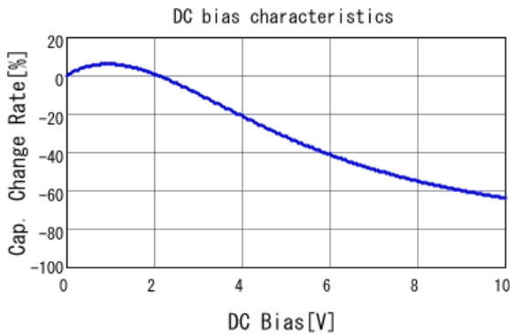
■ GRM21BR71A475KA73 C-DC bias capchange, 25.0degC, AC1.
