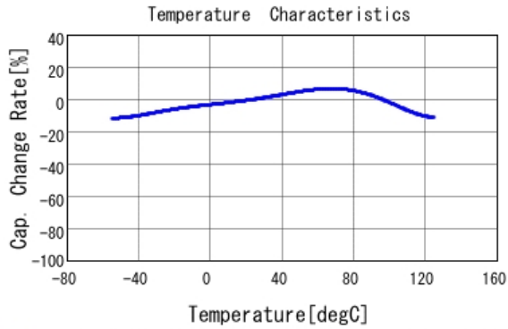
■ GRM21BR71E225KE11 C-Temp. capchange, DC0.0V, AC0.8Vrm
