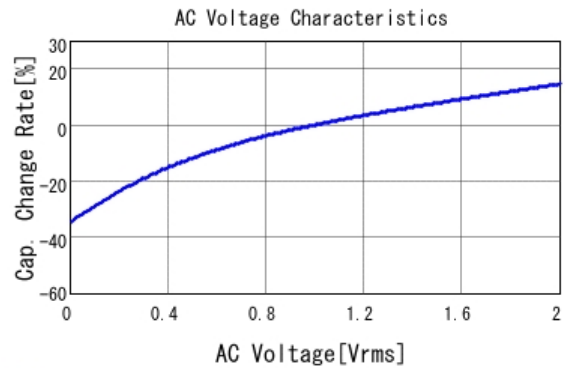
■ GRM21BR71E225KE11 C-AC Voltage capchange, DCOV, 25.0d
