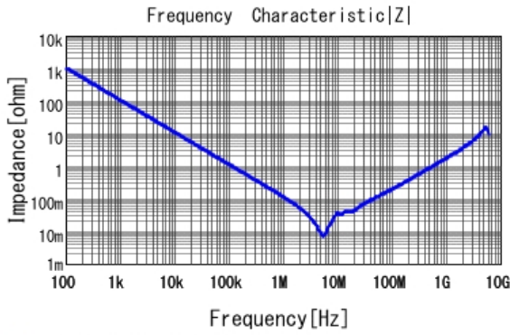
■ GRM21BR71E225KE11 |Z| DCOV, 25degC
