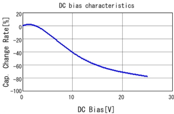
■ GRM21BR71E225KE11 C-DC bias capchange, 25.0degC, AC1V
