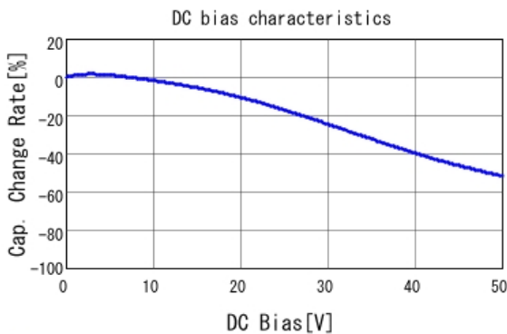
■ GRM21BR71H224KA01 C-DC bias capchange, 25.0degC, AC1.
