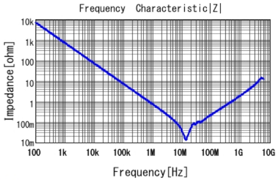
■ GRM21BR71H224KA01 |Z| DCOV, 25degC
