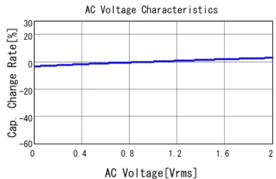
■ GRM21BR71H224KA01 C-AC Voltage capchange, DCOV, 25.0d
