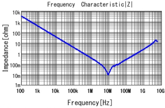
■ GRM21BR71H474KA88 |Z| DCOV, 25degC
