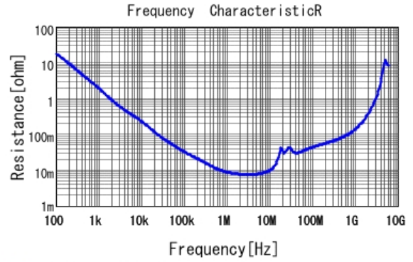
■ GRM21BR71H474KA88 R DCOV, 25degC
