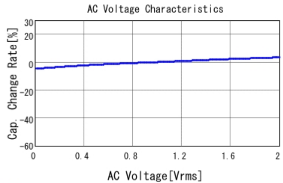
■ GRM21BR71H474KA88 C-AC Voltage capchange, DCOV, 25.0d
