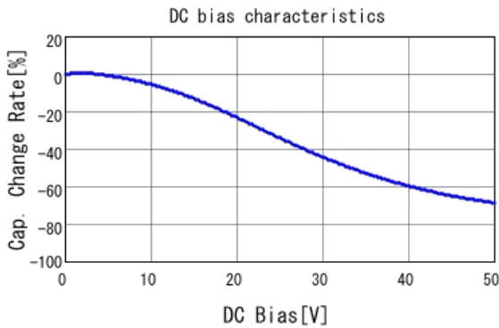
■ GRM21BR71H474KA88 C-DC bias capchange, 25.0degC, AC1.
