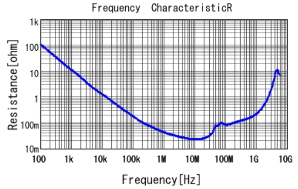
■ GRM21BR71H683KA01 R DCOV, 25degC
