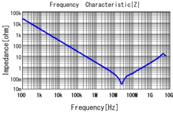
■ GRM21BR71H683KA01 |Z| DCOV, 25degC
