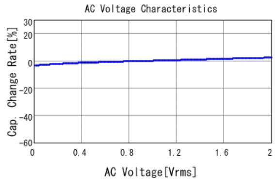
■ GRM21BR71H683KA01 C-AC Voltage capchange, DCOV, 25.0d
