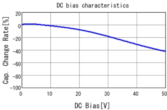
■ GRM21BR71H683KA01 C-DC bias capchange, 25.0degC, AC1.
