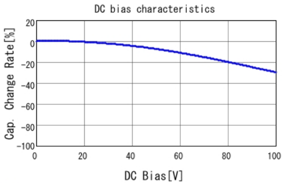
■ GRM21BR72A103KA01 C-DC bias capchange, 25.0degC, AC1.
