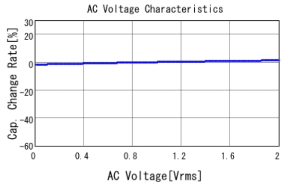
■ GRM21BR72A103KA01 C-AC Voltage capchange, DCOV, 25.0d
