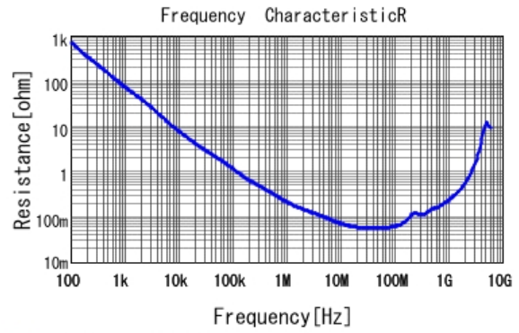
■ GRM21BR72A103KA01 R DCOV, 25degC
