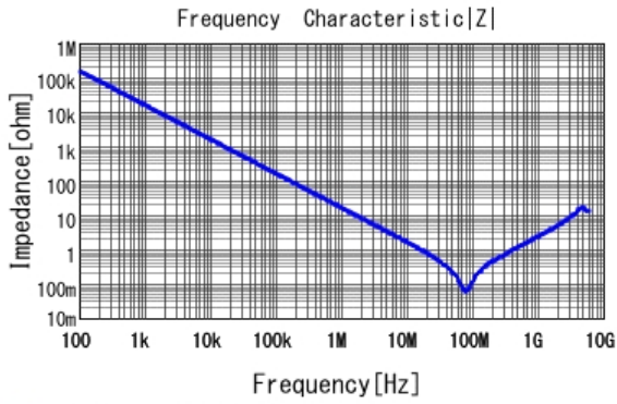
■ GRM21BR72A103KA01 |Z| DCOV, 25degC
