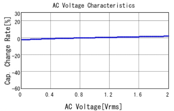
■ GRM21BR72A333KA01 C-AC Voltage capchange, DCOV, 25.0d
