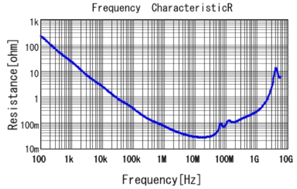
■ GRM21BR72A333KA01 R DCOV, 25degC
