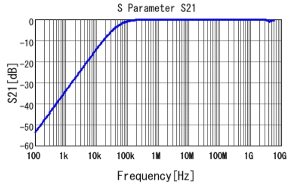
■ GRM21BR72A333KA01 S21 DC0V, 25degC
