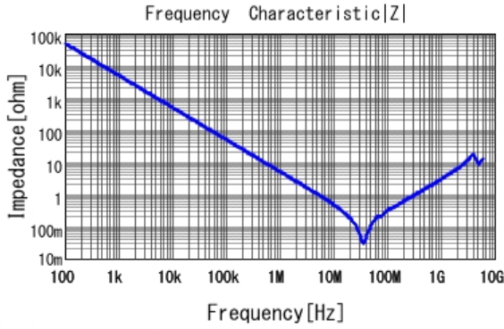
■ GRM21BR72A333KA01 |Z| DCOV, 25degC
