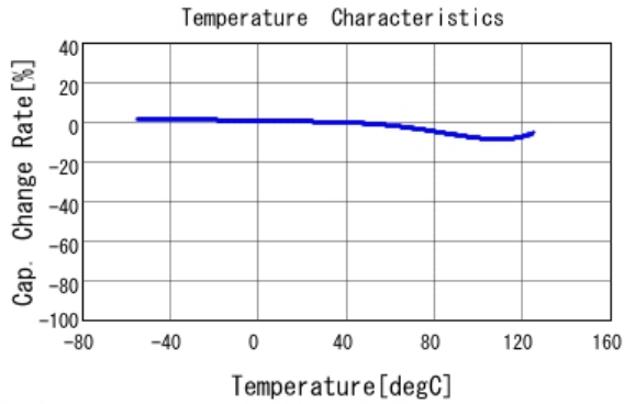
■ GRM21BR72A333KA01 C-Temp. capchange, DC0.0V, AC1.0V rm
