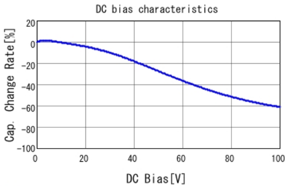
■ GRM21BR72A333KA01 C-DC bias capchange, 25.0degC, AC1.
