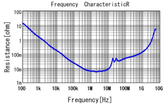
■ GRM21BR72A474KA73 R DCOV, 25degC
