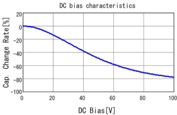
■ GRM21BR72A474KA73 C-DC bias capchange, 25.0degC, AC1.
