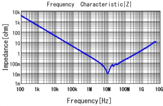
■ GRM21BR72A474KA73 |Z| DCOV, 25degC
