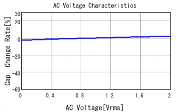
■ GRM21BR72A474KA73 C-AC Voltage capchange, DCOV, 25.0d
