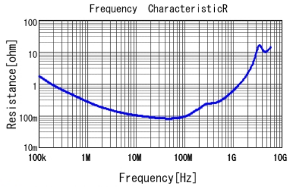
■ GRM21BR72E103KW03 R DCOV, 25degC
