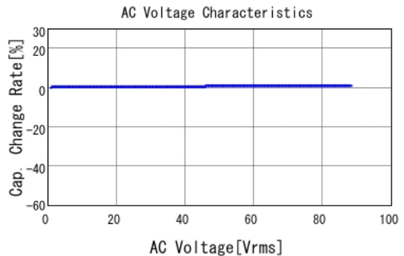
■ GRM21BR72E103KW03 C-AC Voltage capchange, DCOV, 25.0d
