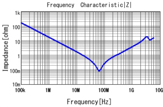
■ GRM21BR72E103KW03 |Z| DCOV, 25degC
