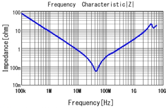
■ GRM21BR72E223KW03 |Z| DCOV, 25degC
