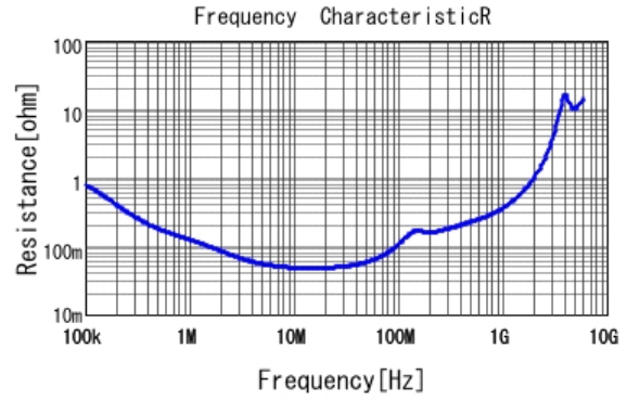
■ GRM21BR72E223KW03 R DCOV, 25degC
