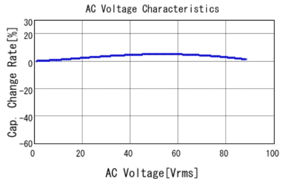
■ GRM21BR72E223KW03 C-AC Voltage capchange, DCOV, 25.0d
