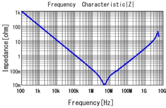
■ GRM316B31E225KA75 |Z| DCOV, 20degC
