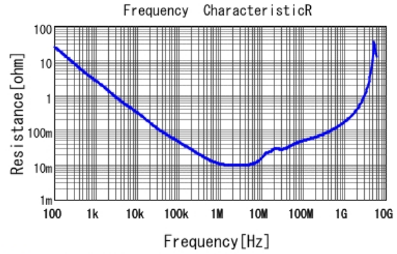
■ GRM316B31E225KA75 R DCOV, 20degC
