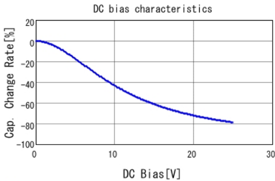
■ GRM316B31E225KA75 C-DC bias capchange, 20.0degC, AC1.
