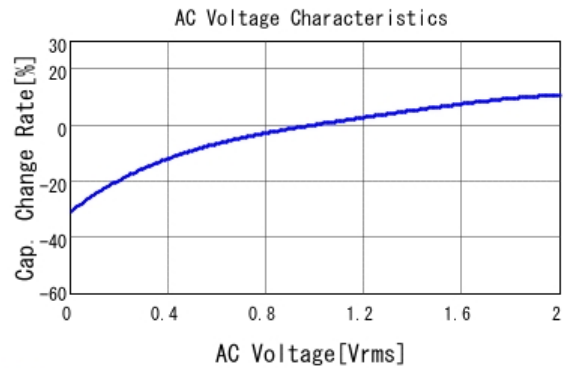
■ GRM316B31E225KA75 C-AC Voltage capchange, DCOV, 20.0d
