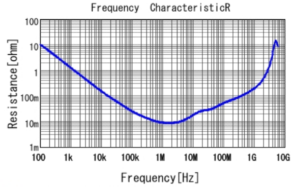
■ GRM316R61A475KE19 R DCOV, 25degC
