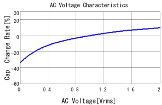
■ GRM316R61A475KE19 C-AC Voltage capchange, DCOV, 25.0d
