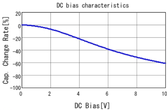
■ GRM316R61A475KE19 C-DC bias capchange, 25.0degC, AC1.
