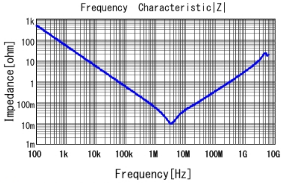
■ GRM316R61A475KE19 |Z| DCOV, 25degC
