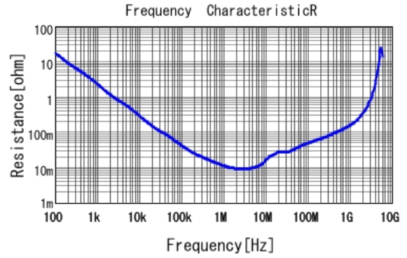
■ GRM316R61C225KA88 R DCOV, 25degC
