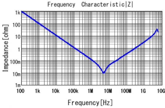
■ GRM316R61C225KA88 |Z| DCOV, 25degC
