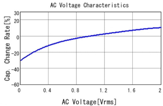
■ GRM316R61C225KA88 C-AC Voltage capchange, DCOV, 25.0d
