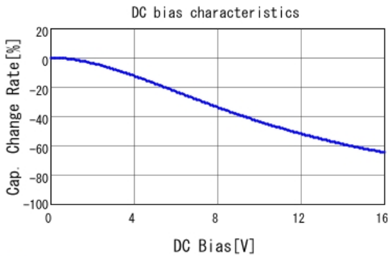
■ GRM316R61C225KA88 C-DC bias capchange, 25.0degC, AC1.
