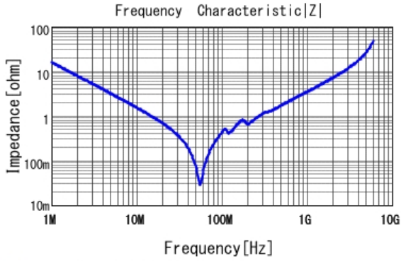
■ GRM3195C1H103JA01 |Z| DCOV, 25degC
