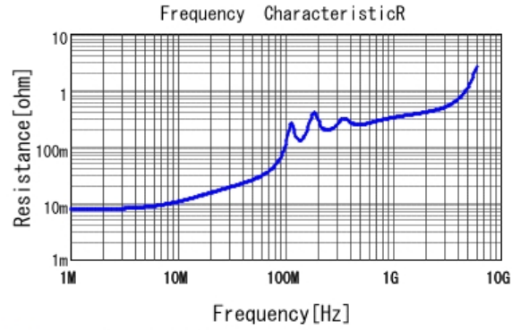
■ GRM3195C1H103JA01 R DCOV, 25degC
