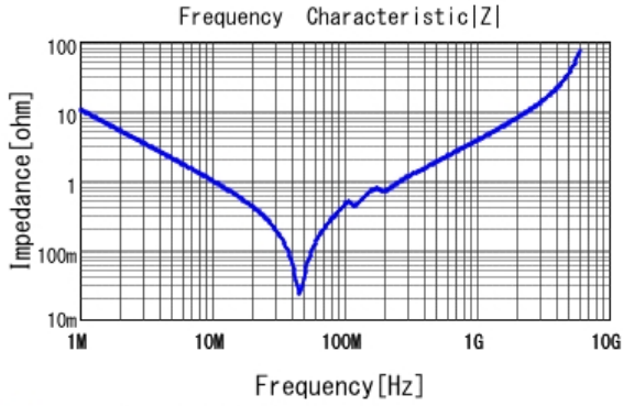
■ GRM3195C1H153JA01 |Z| DCOV, 25degC
