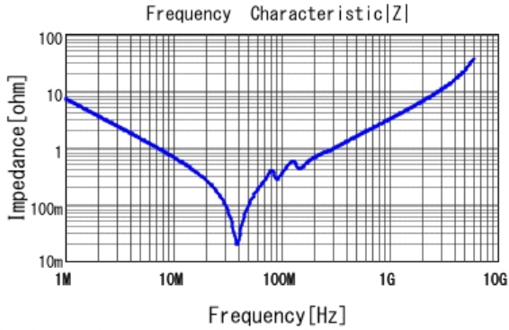
■ GRM3195C1H223JA01 |Z| DCOV, 25degC
