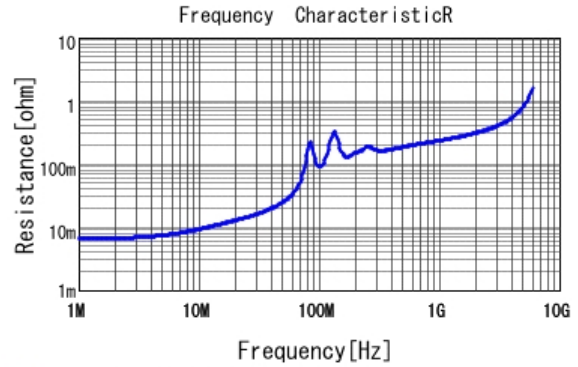
■ GRM3195C1H223JA01 R DCOV, 25degC
