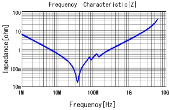
■ GRM3195C1H273JA01 |Z| DCOV, 25degC
