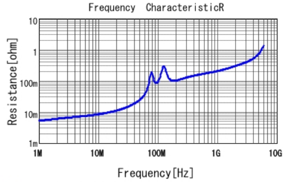
■ GRM3195C1H273JA01 R DCOV, 25degC
