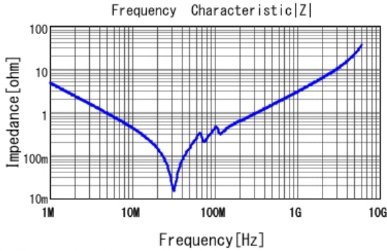
■ GRM3195C1H333JA01 |Z| DCOV, 25degC
