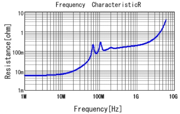
■ GRM3195C1H333JA01 R DCOV, 25degC
