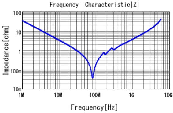
■ GRM3195C1H472JA01 |Z| DCOV, 25degC
