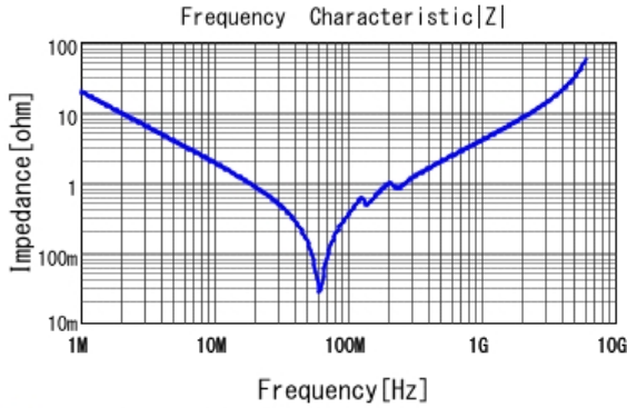
■ GRM3195C1H822JA01 |Z| DCOV, 25degC
