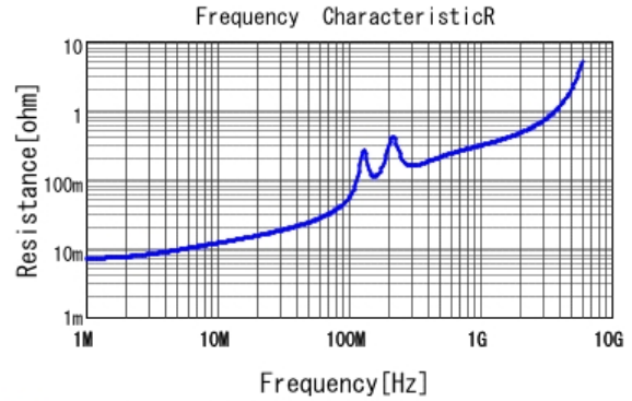
■ GRM3195C1H822JA01 R DCOV, 25degC
