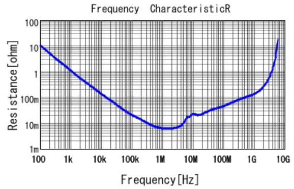
■ GRM319R61A475KA01 R DCOV, 25degC
