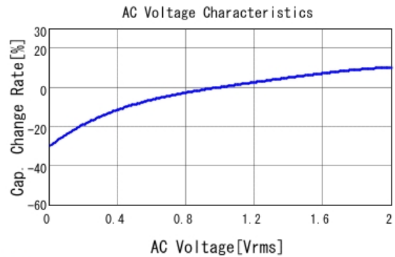
■ GRM319R61A475KA01 C-AC Voltage capchange, DCOV, 25.0d
