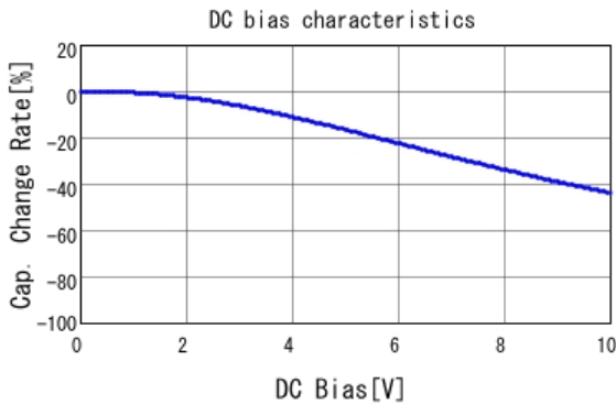
■ GRM319R61A475KA01 C-DC bias capchange, 25.0degC, AC1.
