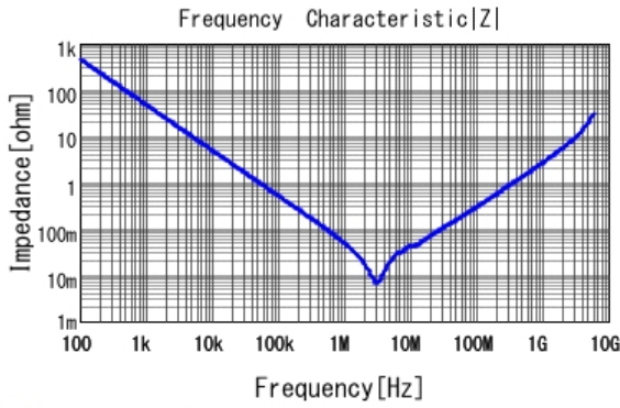
■ GRM319R61A475KA01 |Z| DCOV, 25degC
