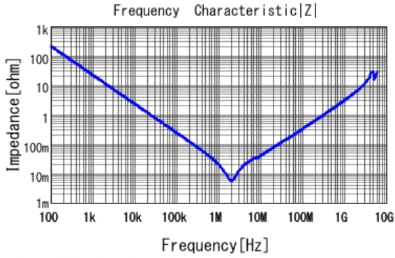
■ GRM319R61C106KE15 |Z| DCOV, 25degC
