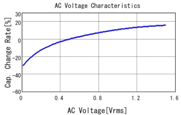
■ GRM319R61C106KE15 C-AC Voltage capchange, DCOV, 25.0d
