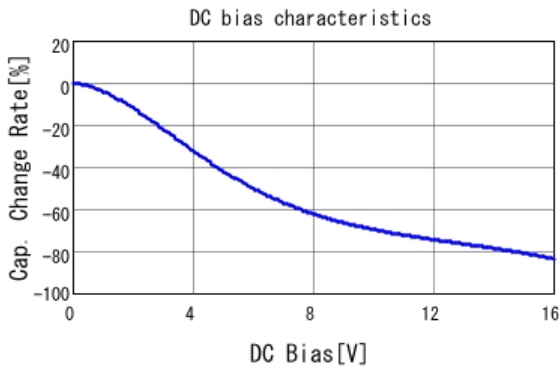
■ GRM319R61C106KE15 C-DC bias capchange, 25.0degC, AC0.
