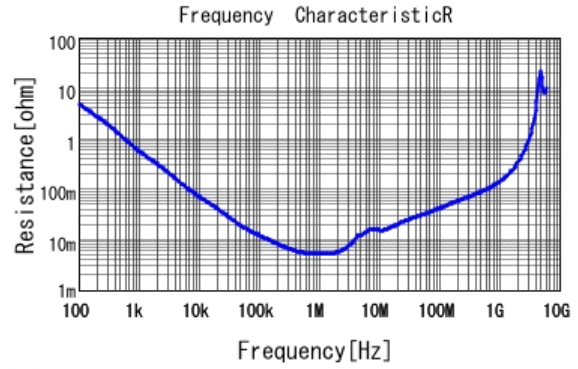
■ GRM319R61C106KE15 R DCOV, 25degC
