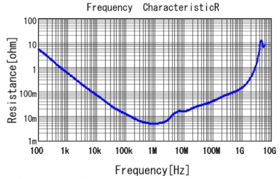
■ GRM319R61E106KA12 R DCOV, 25degC
