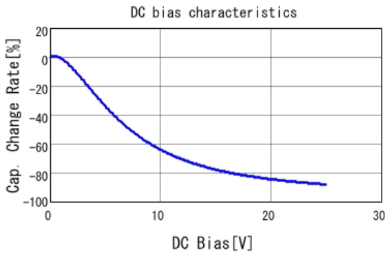
■ GRM319R61E106KA12 C-DC bias capchange, 25.0degC, AC1.
