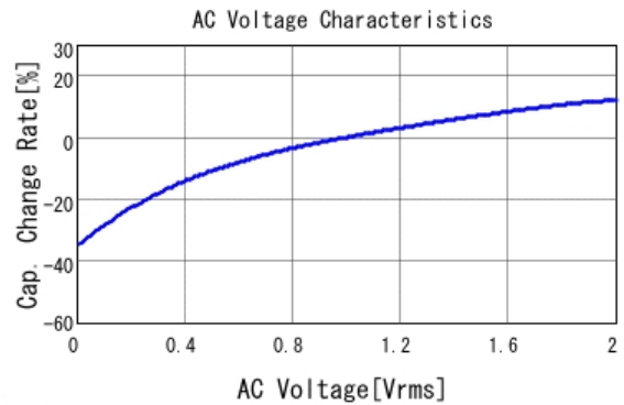
■ GRM319R61H475KA12 C-AC Voltage capchange, DCOV, 25.0d
