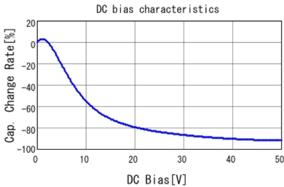
■ GRM319R61H475KA12 C-DC bias capchange, 25.0degC, AC1.
