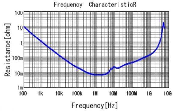
■ GRM319R61H475KA12 R DCOV, 25degC
