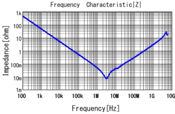
■ GRM319R61H475KA12 |Z| DCOV, 25degC
